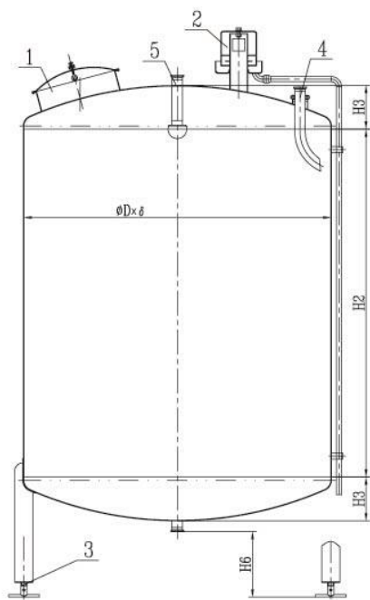
Upper dish shape and lower dish shape
