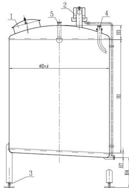
Upper dish shape and lower inclined bottom
