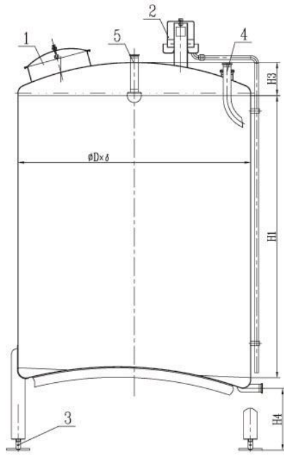
Upper dish shape and lower convex shape
